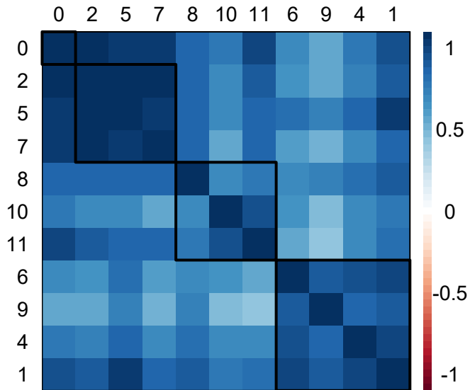
Stochastic block model GCM
