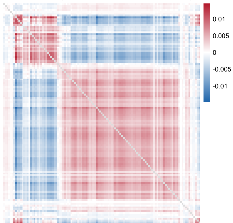
EBF: rank 2 (StARS-selected lambda = 0.253)
