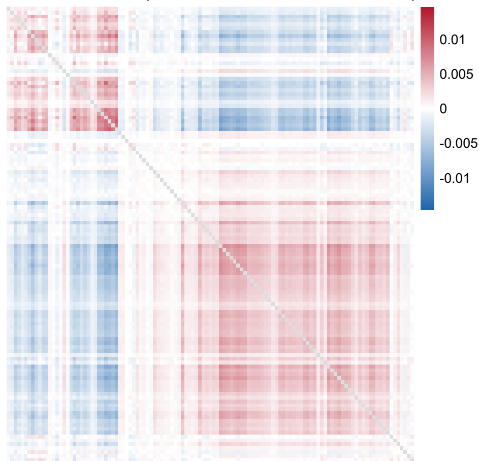
non-EBF: rank 2 (StARS-selected lambda = 0.323)
