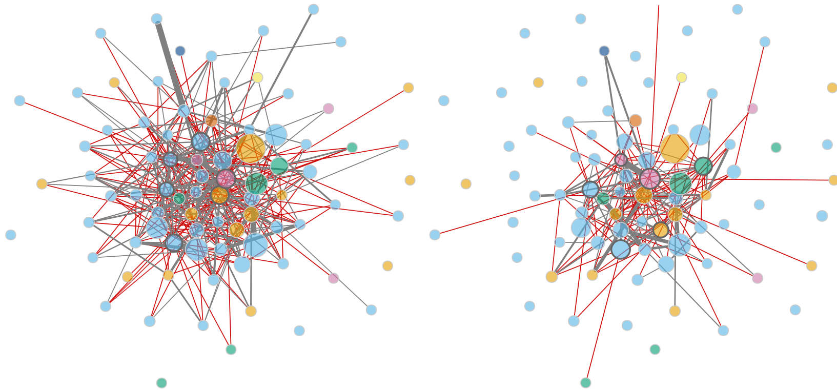
SPIEC-EASI MB with BayesMultRepl
