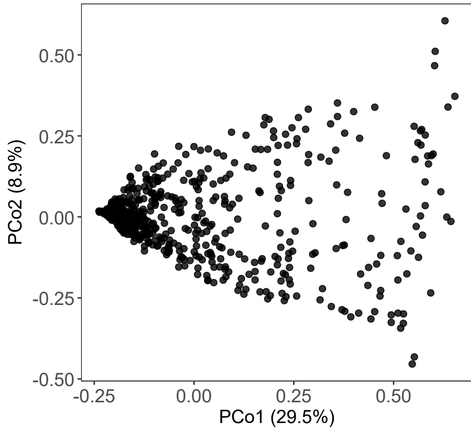
Bray-Curtis dissimilarity
