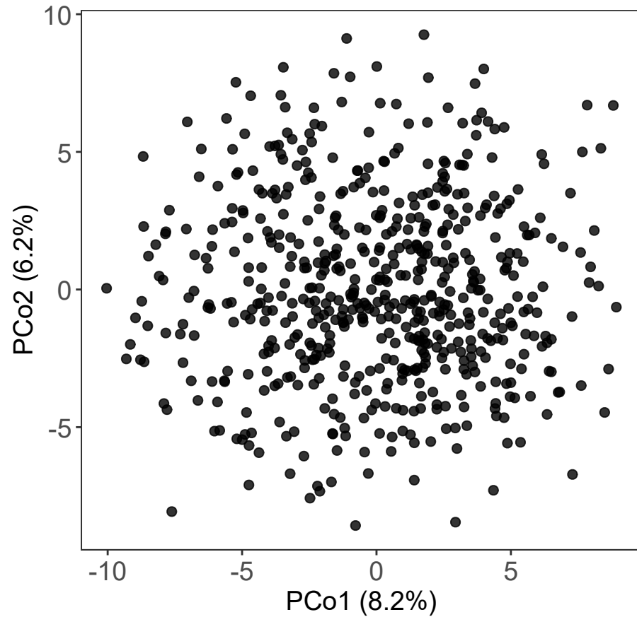
Aitchison distance
