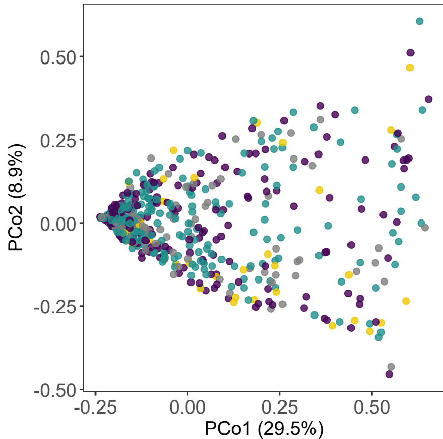
Bray-Curtis dissimilarity: Siblings
