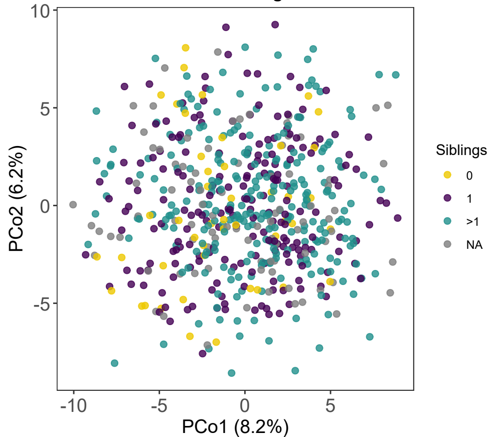
Aitchison distance: Siblings
