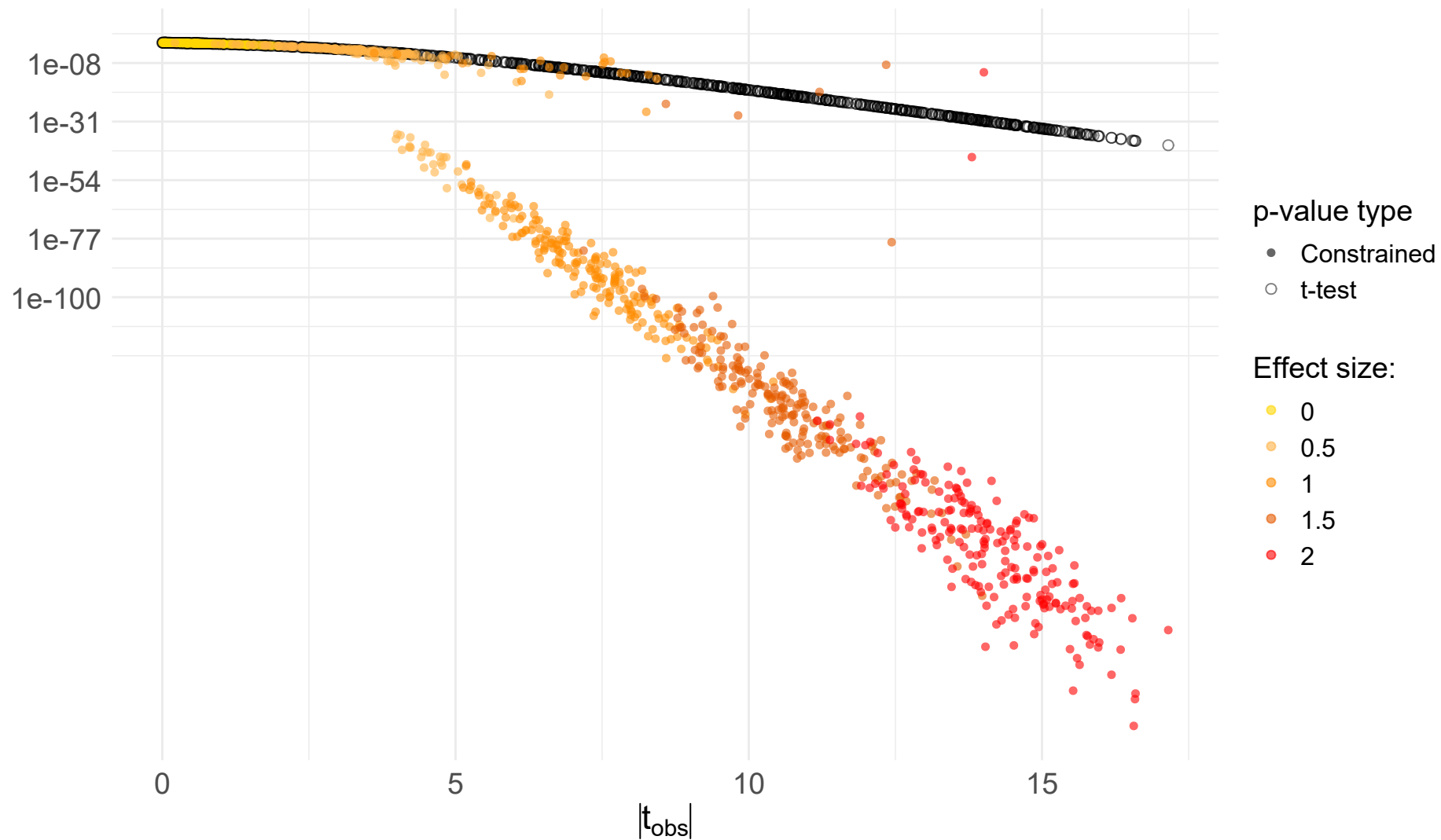
t-test vs. permApprox constrained (all test, eps = 0)
