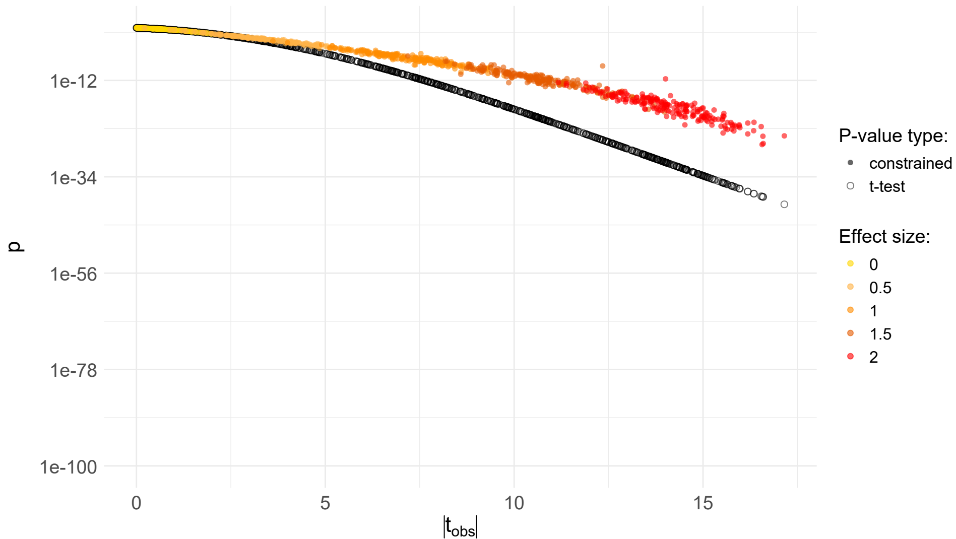
t-test vs. permApprox constrained (max test, eps_fact = 0.3)
