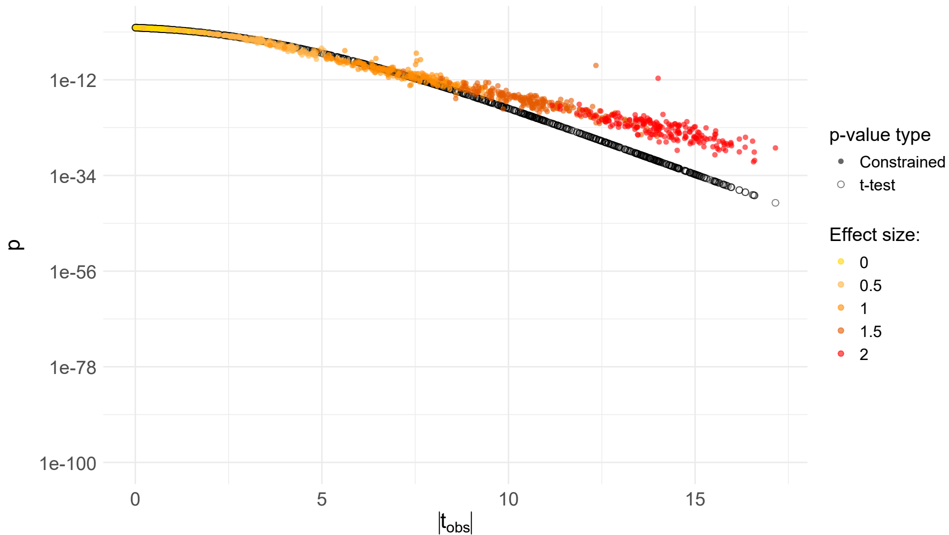
t-test vs. permApprox constrained (all test, eps_fact = 0.2)
