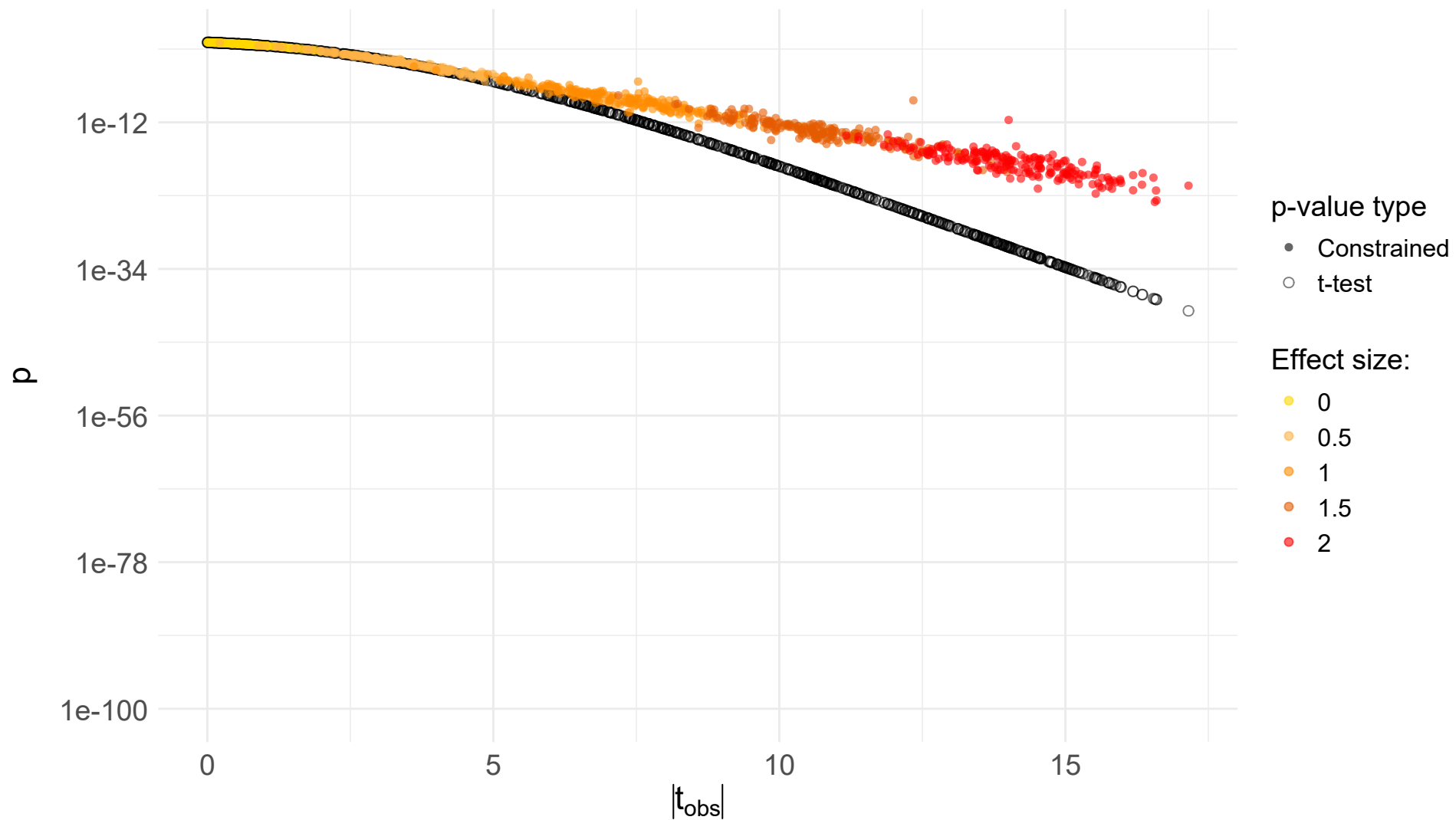
t-test vs. permApprox constrained (all test, eps_fact = 0.5)
