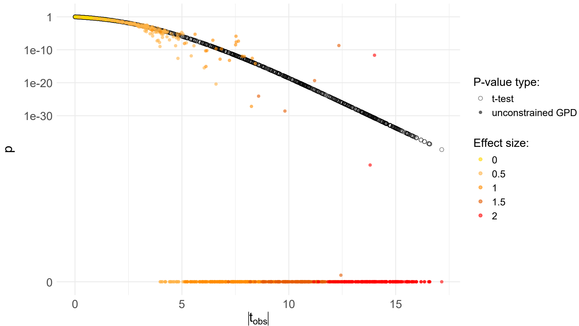
Unconstrained permApprox vs. t-test
