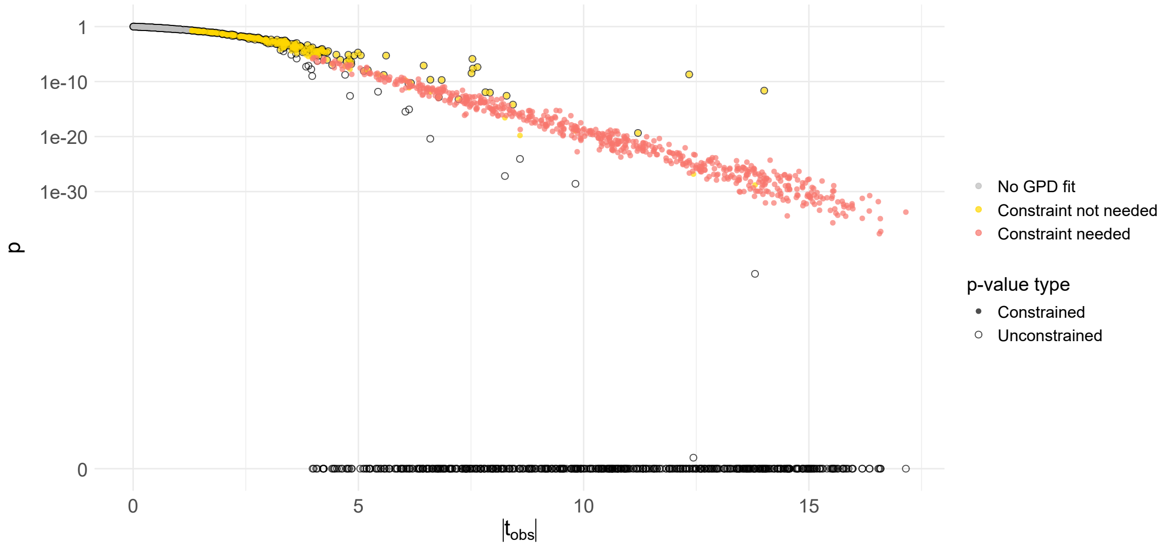
permApprox unconstrained vs. constrained (all, eps = 0.1)
