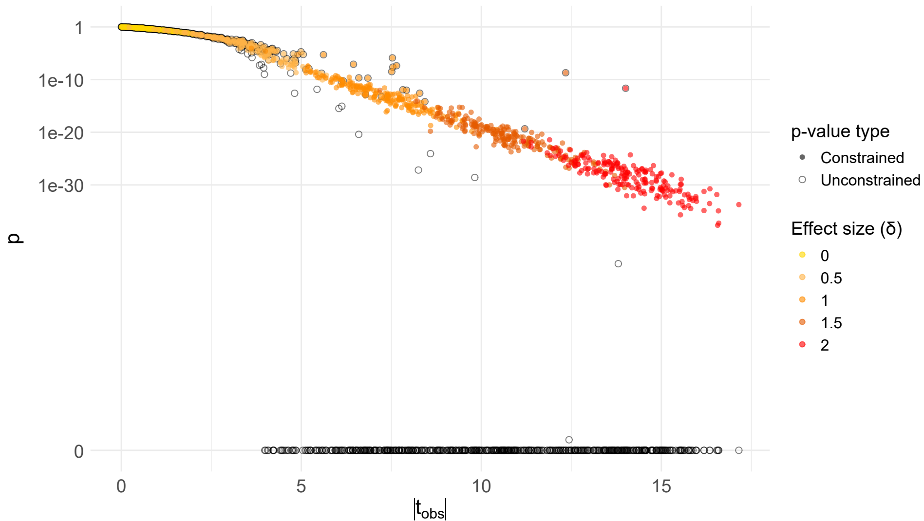
permApprox unconstrained vs. constrained (all tests, eps = 0.1)
