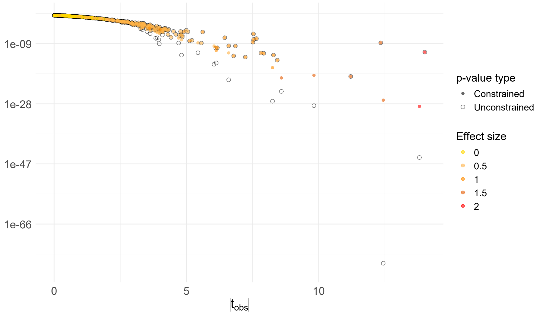
permApprox unconstrained (non-zero only) vs. constrained (all tests, eps = 0.1)
