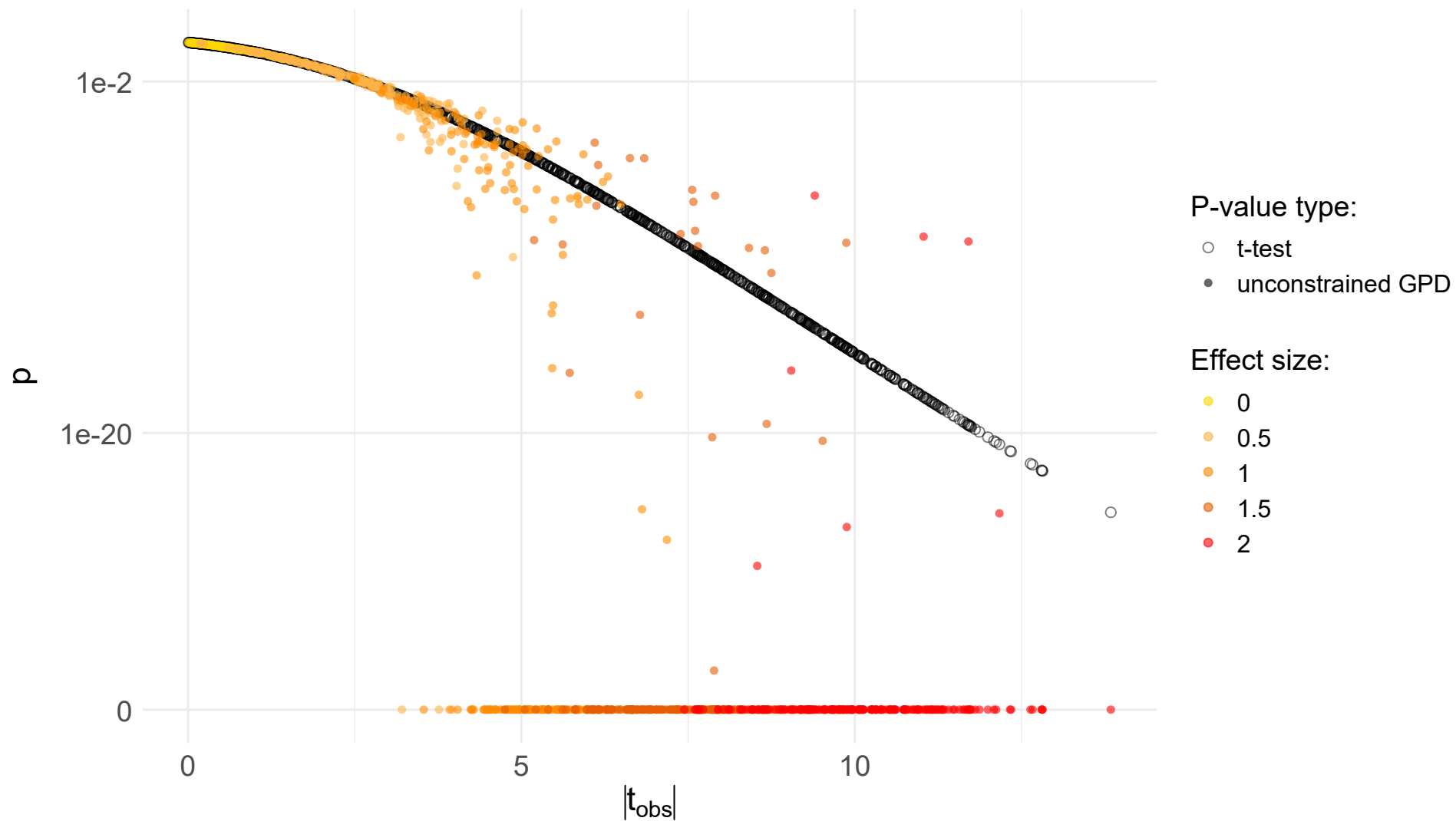
Unconstrained permApprox vs. t-test (n = 50)
