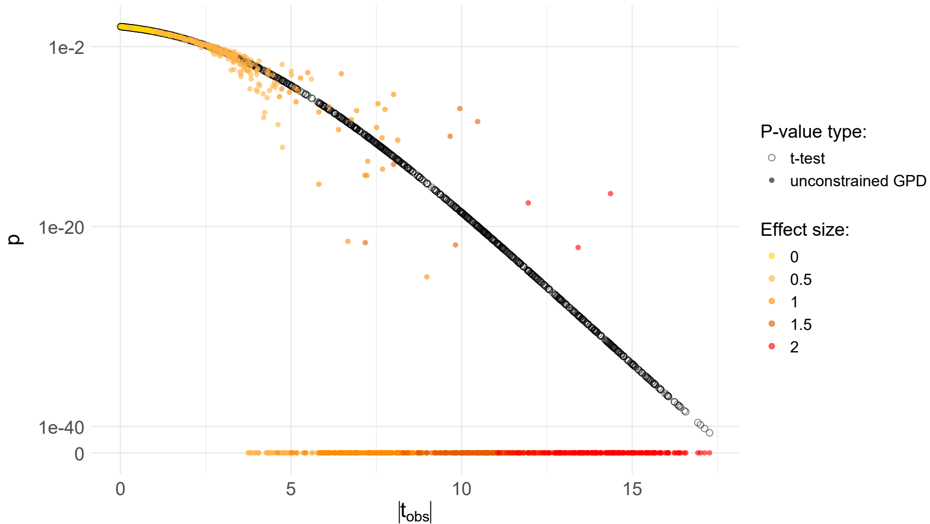
Unconstrained permApprox vs. t-test (n = 100)
