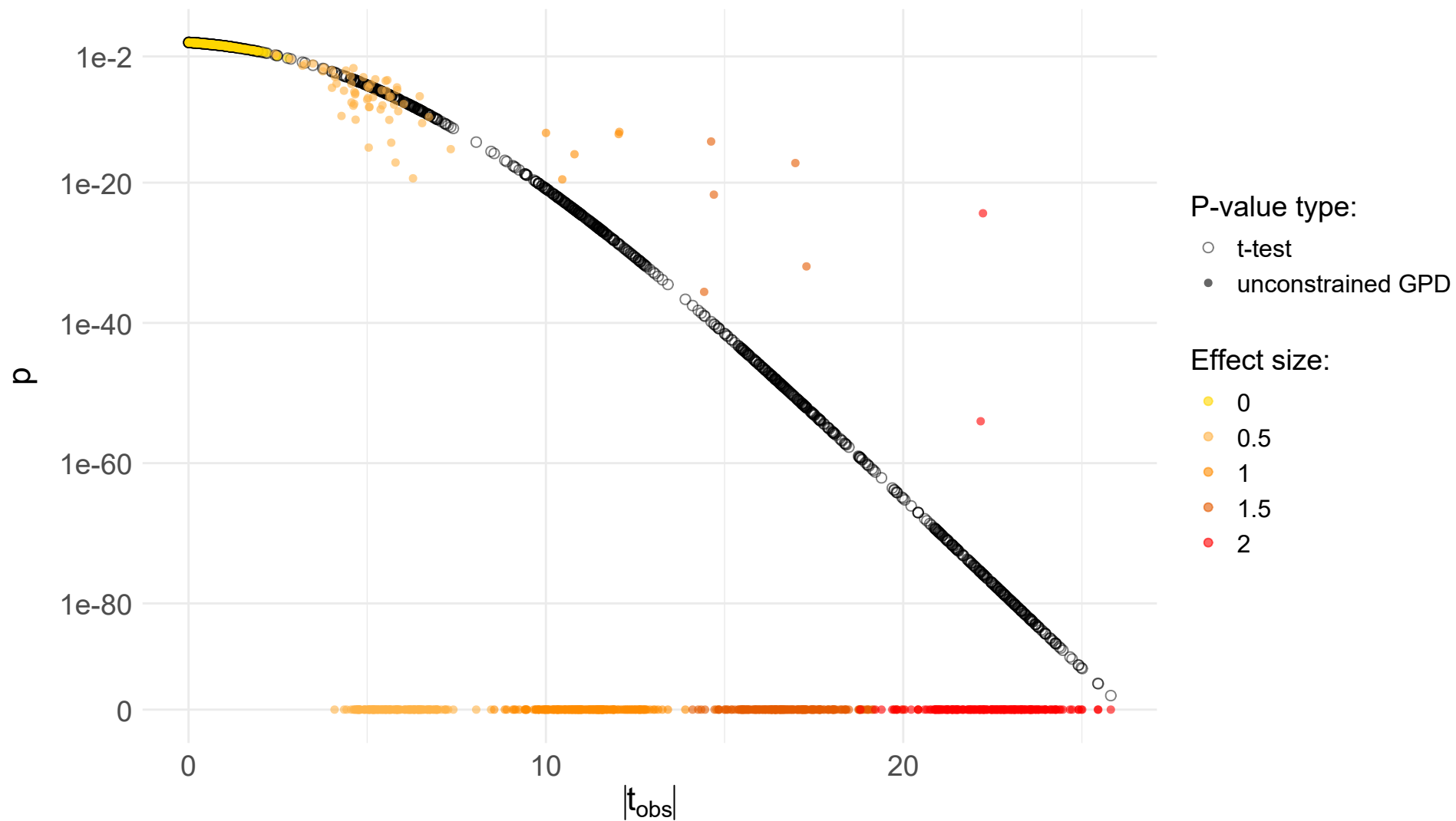
Unconstrained permApprox vs. t-test (n = 250)
