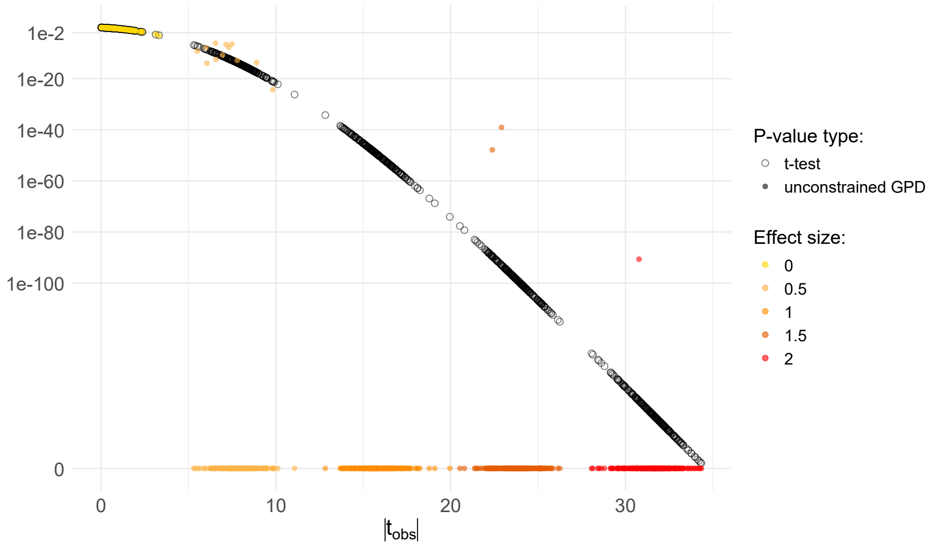
Unconstrained permApprox vs. t-test (n = 500)
