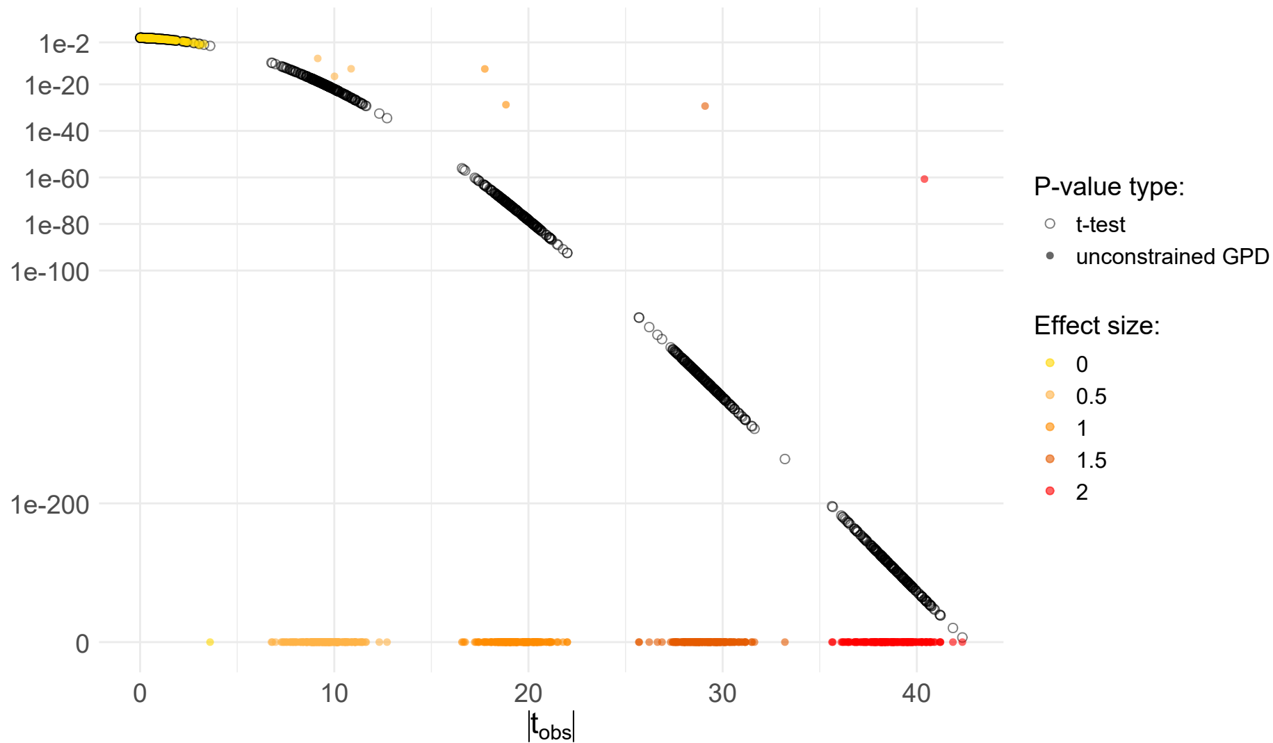
Unconstrained permApprox vs. t-test (n = 750)
