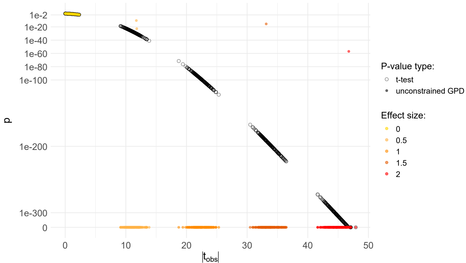
Unconstrained permApprox vs. t-test (n = 1000)
