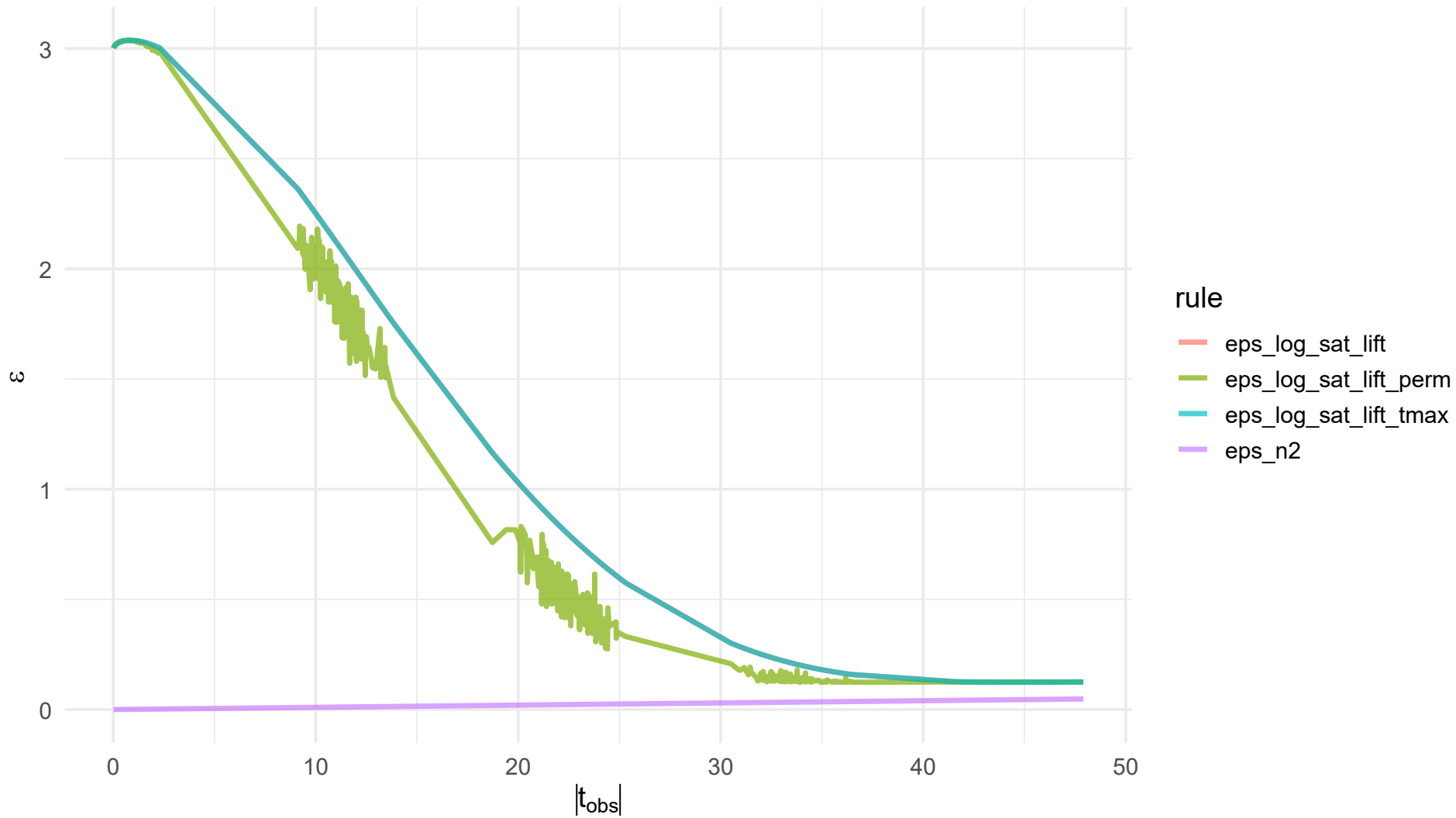
Epsilon scaling comparison (n = 1000)
