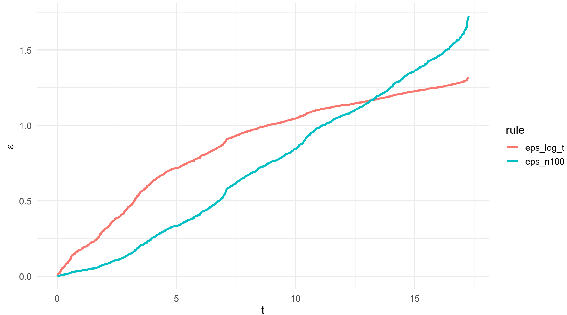
Epsilon scaling comparison
