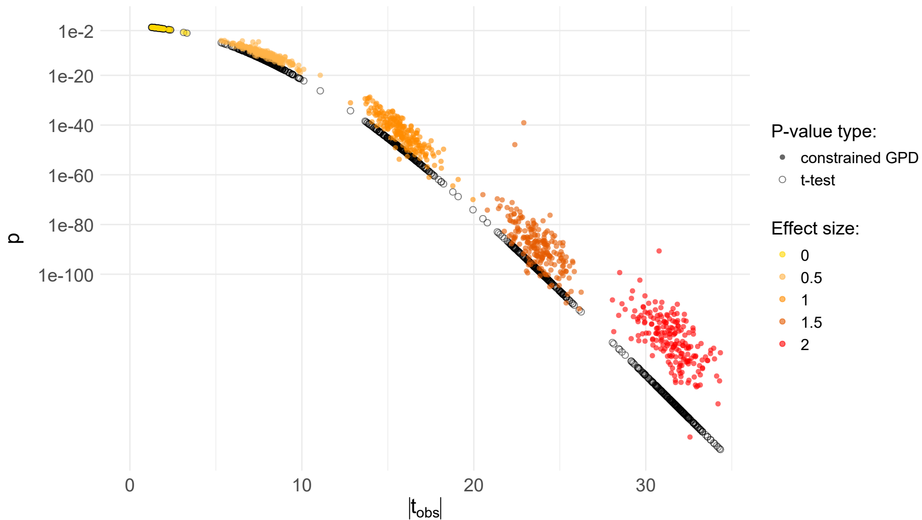
t-test vs. constrained GPD fit (n = 500)
