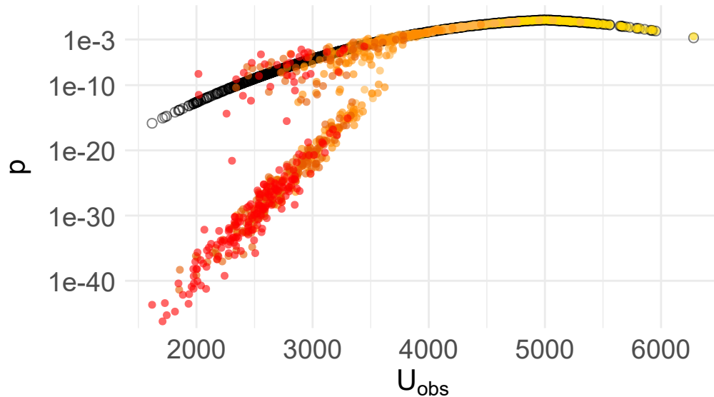
Lifted log-saturation
