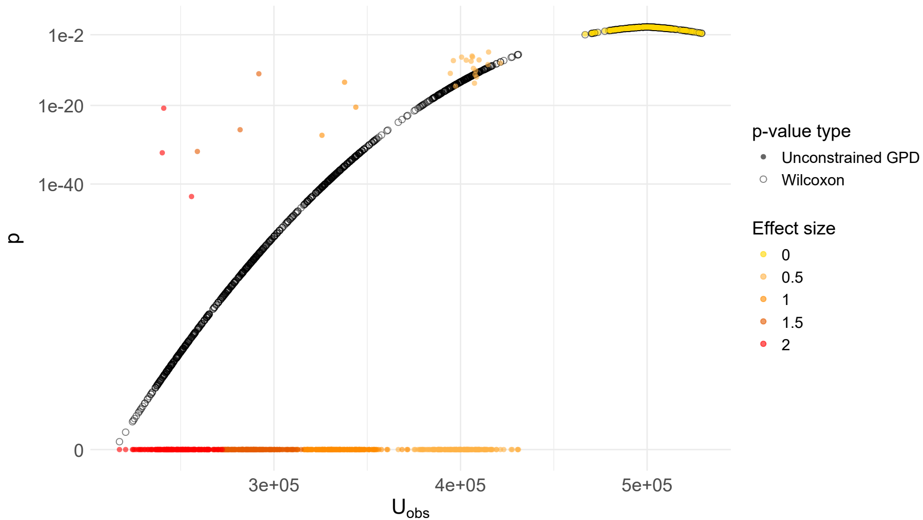
Unconstrained permApprox vs. Mann-Whitney U (n = 1000 )
