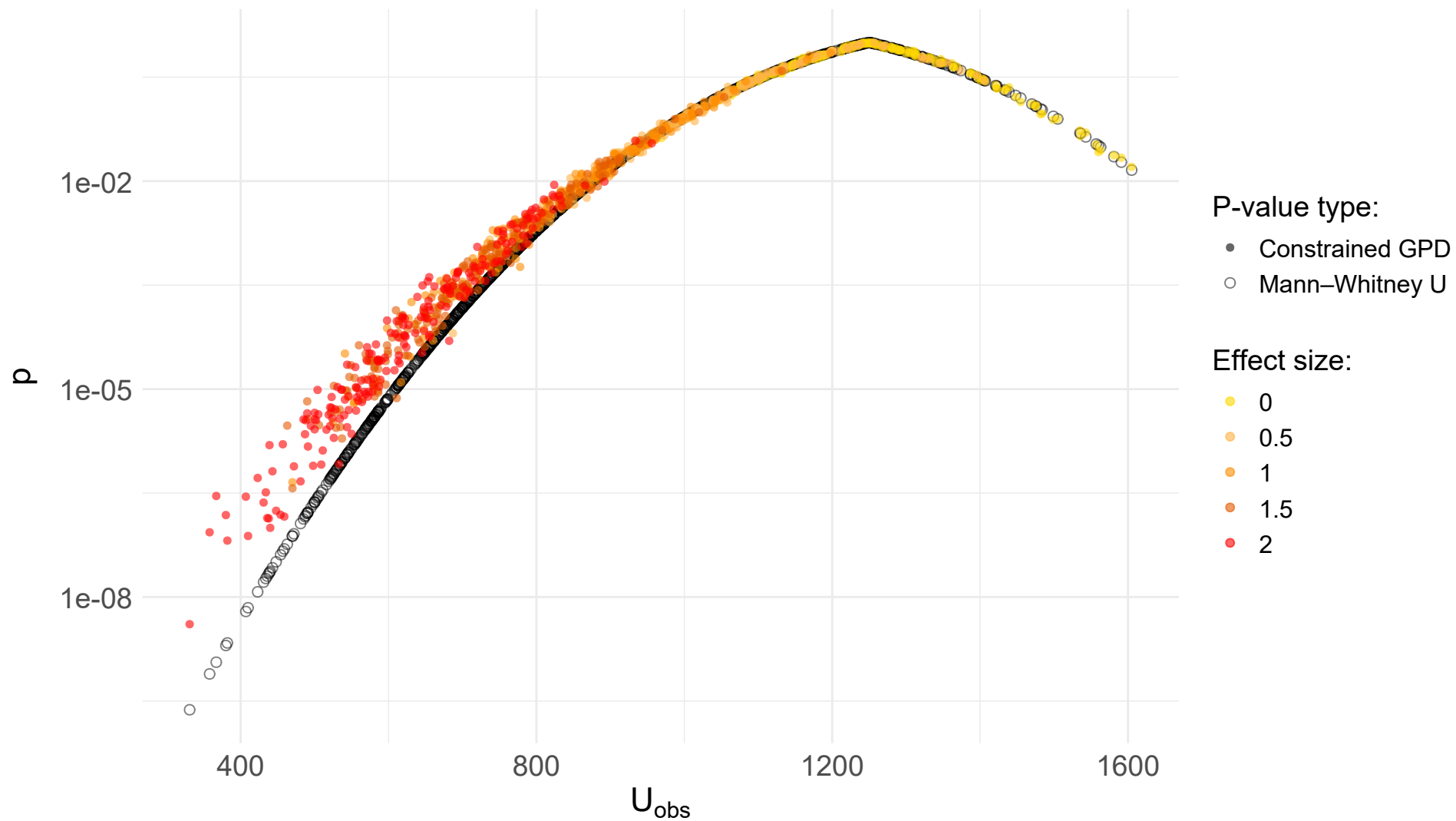
Mann–Whitney U vs. constrained GPD fit (single tests, n = 50 )
