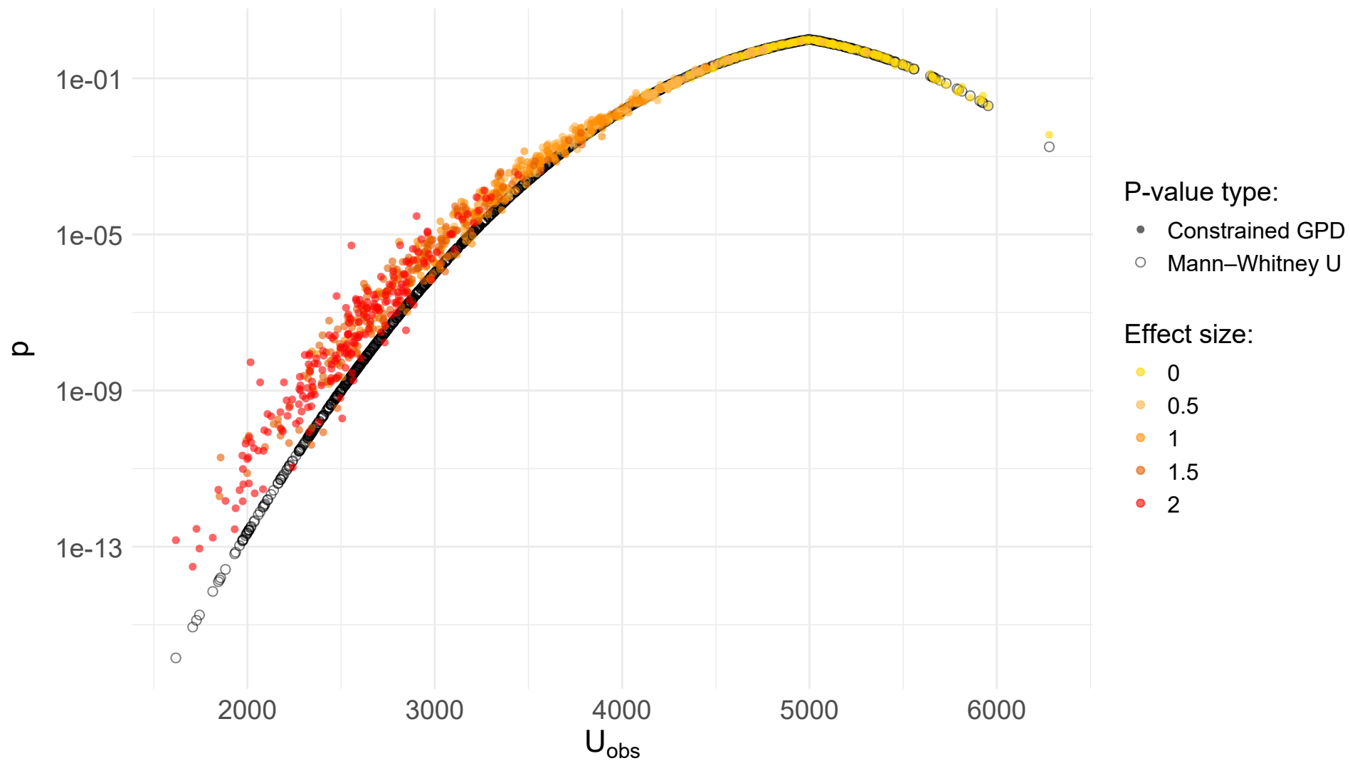
Mann–Whitney U vs. constrained GPD fit (single tests, n = 100 )
