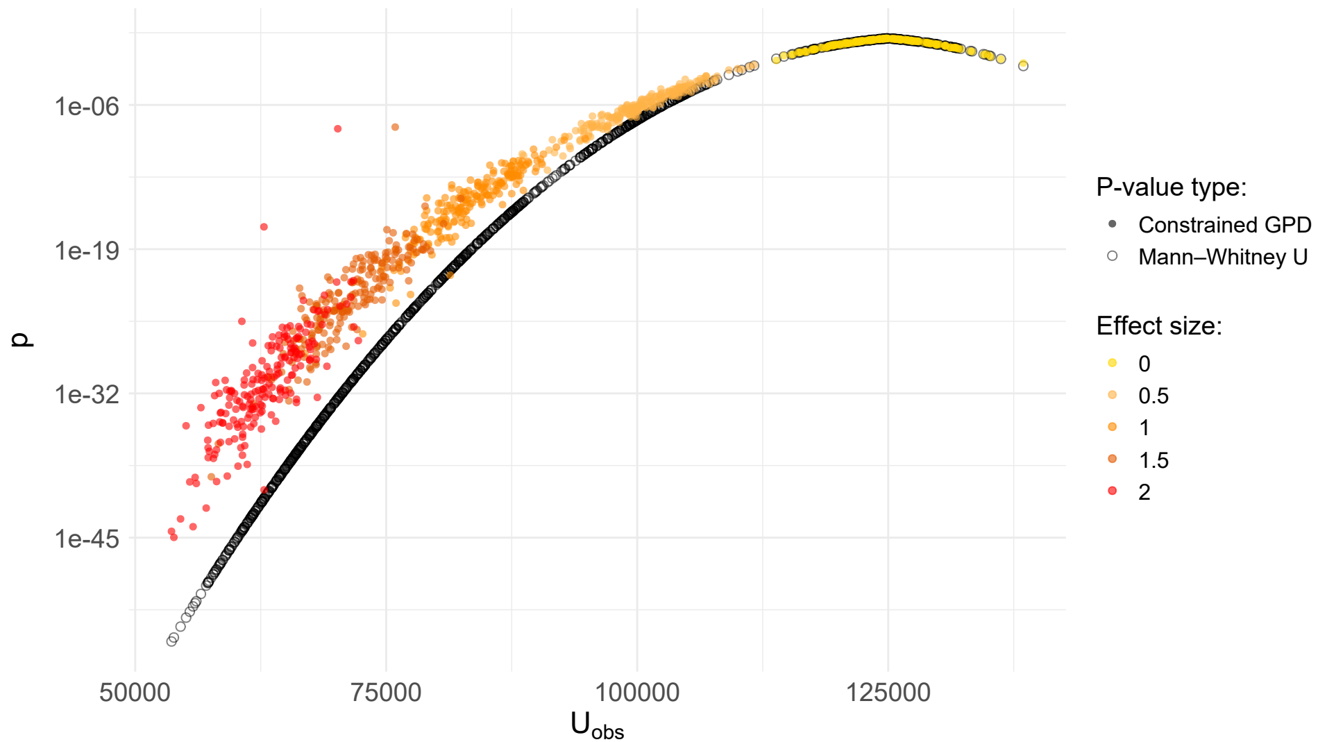
Mann–Whitney U vs. constrained GPD fit (single tests, n = 500)
