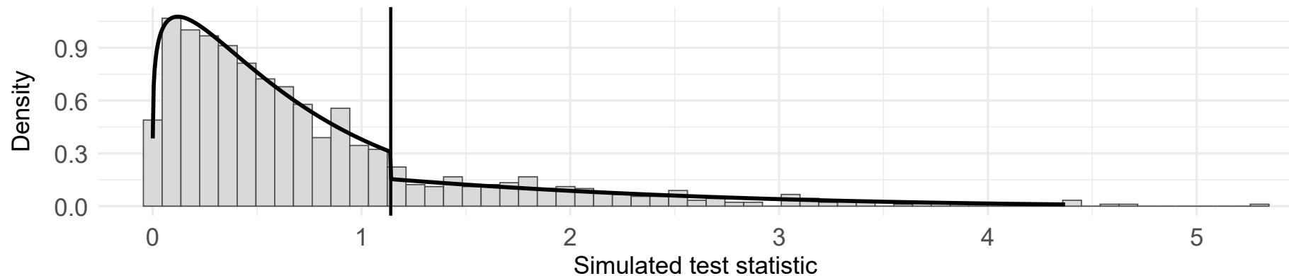
(c) Gamma-GPD ( k_0 = 1000 )
