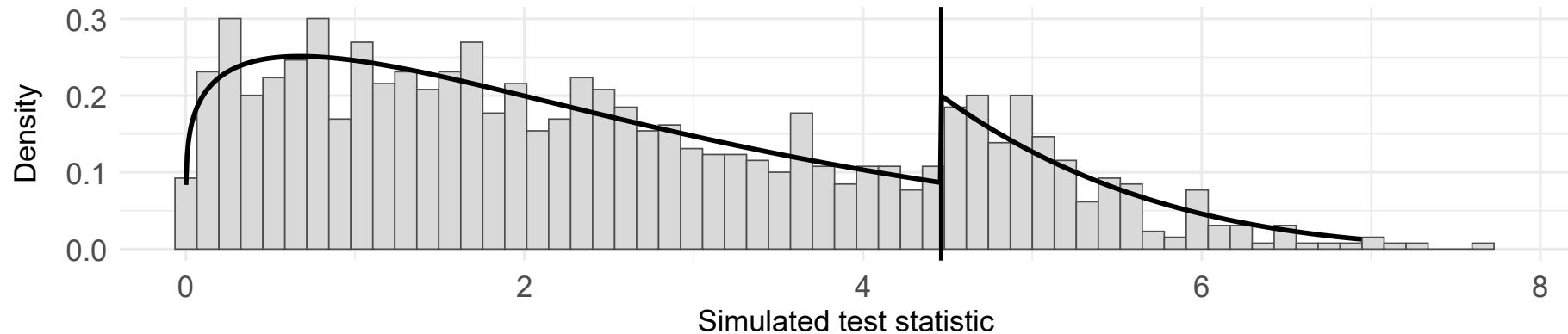
Weibull-GPD ( k_0 = 1000 )
