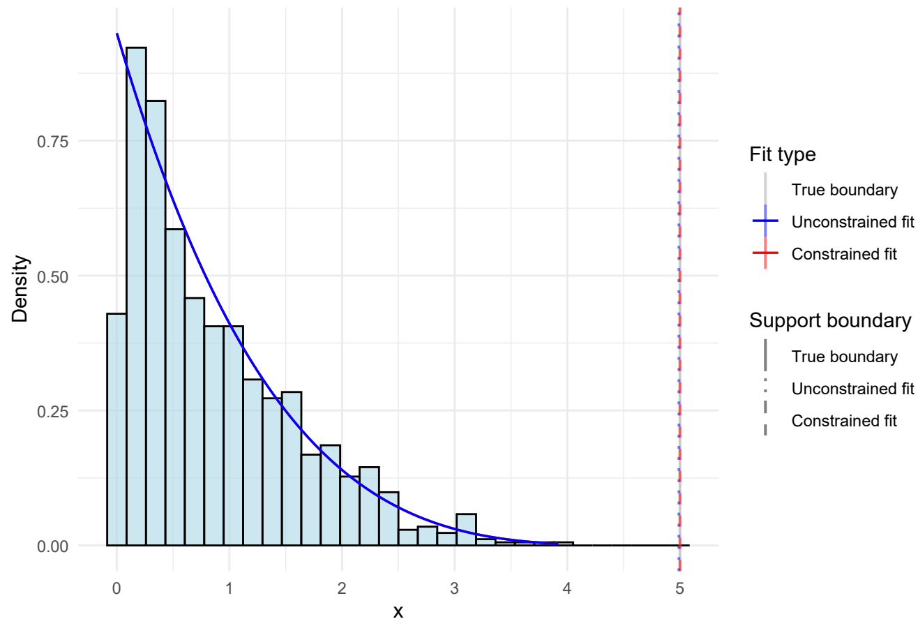
Fitted GPD with bound = 5, shape = -0.2, and scale = 1
