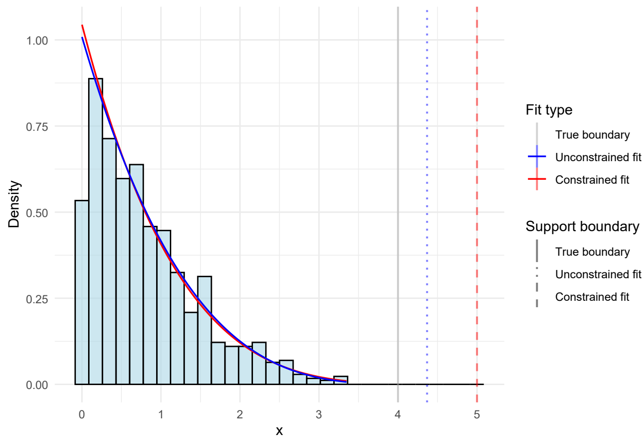
Fitted GPD with bound = 4, shape = -0.25, and scale = 1
