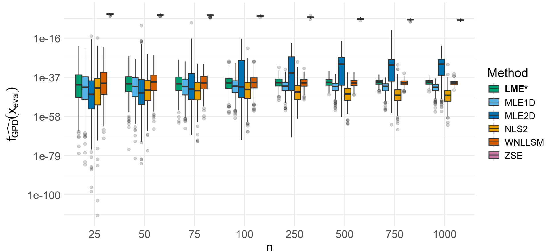
GPD density at evaluation point (constraint active) | \varepsilon = 1
