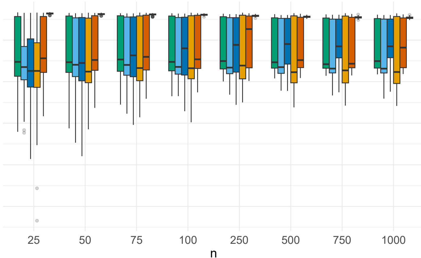
GPD density at evaluation point | \varepsilon = 0
