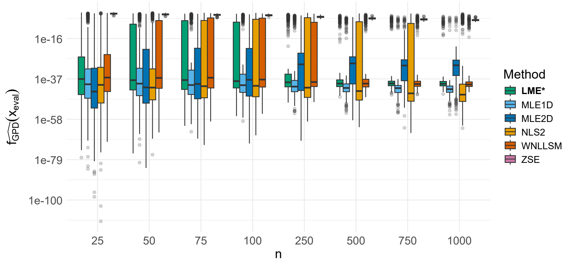
GPD density at evaluation point | \varepsilon = 1
