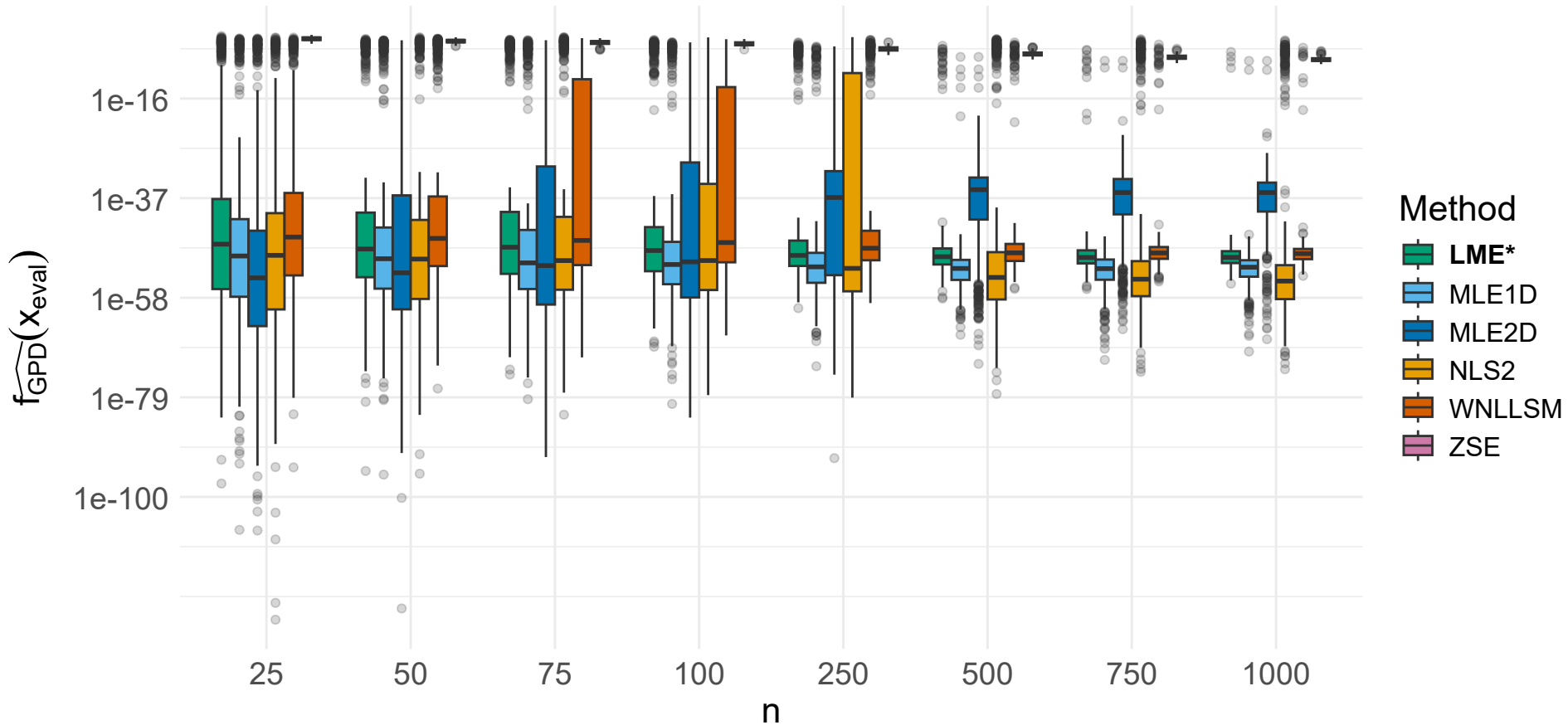
GPD density at evaluation point | \varepsilon = 2
