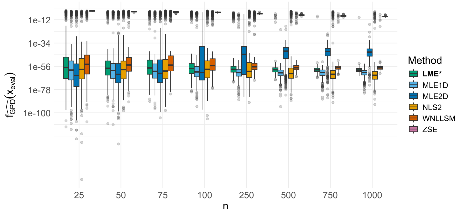
GPD density at evaluation point | \varepsilon = 3
