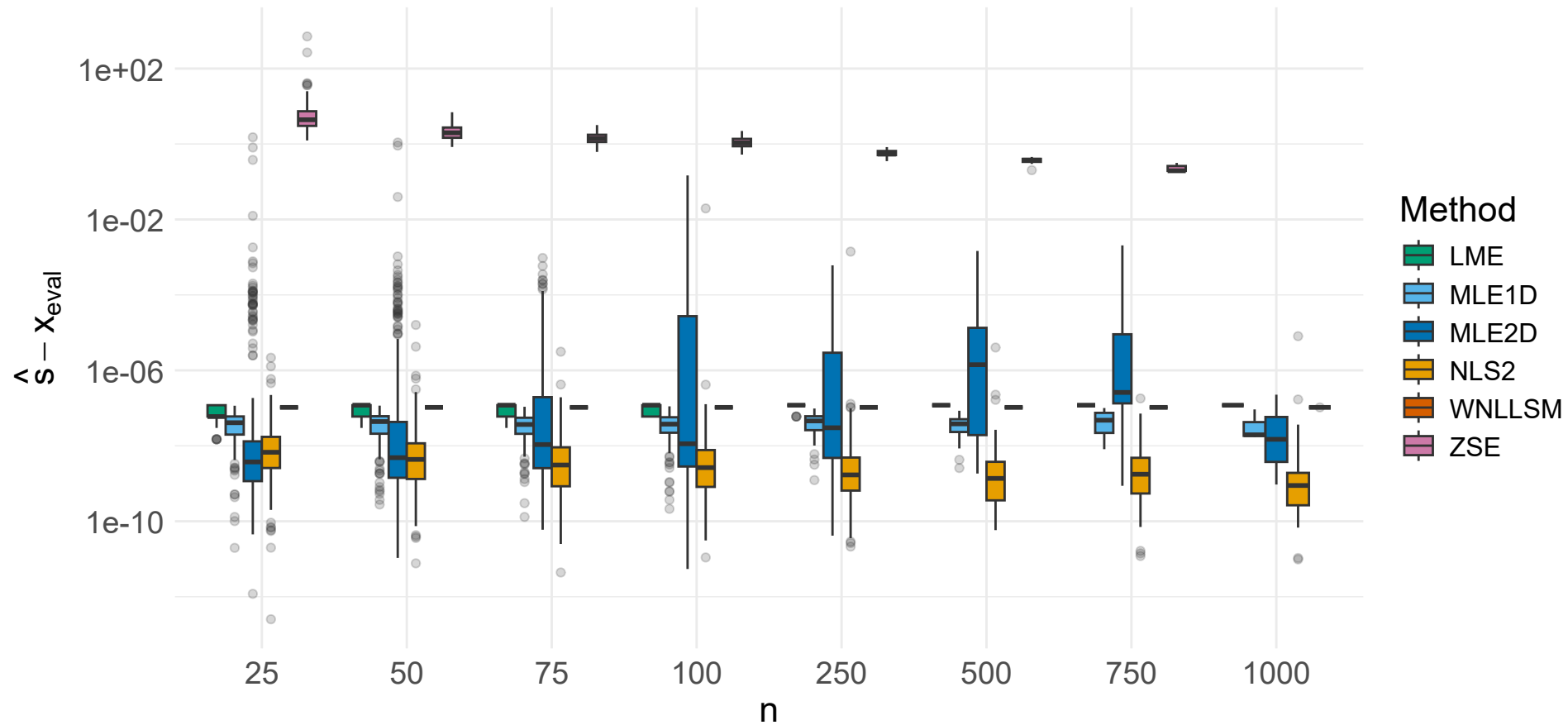
Difference between boundary and eval point (constraint active, log scale) | \varepsilon = -1
