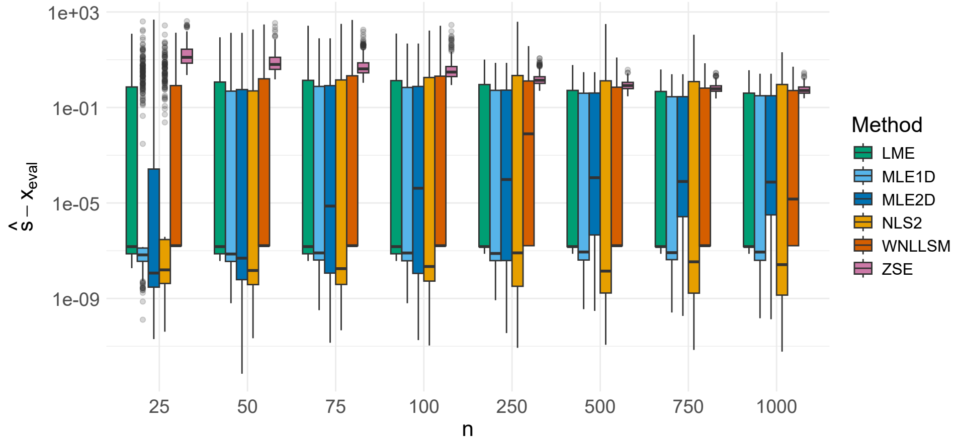
Difference between boundary and eval point (log scale) | \varepsilon = 0
