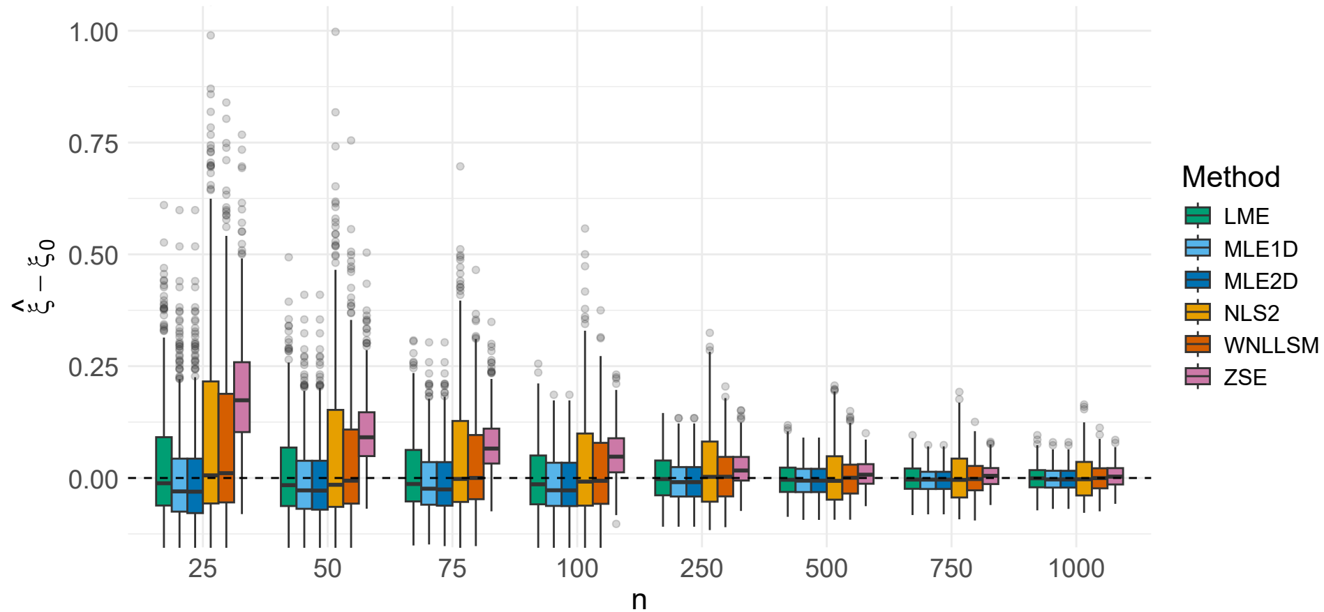
Estimation error in shape | \varepsilon = -1
