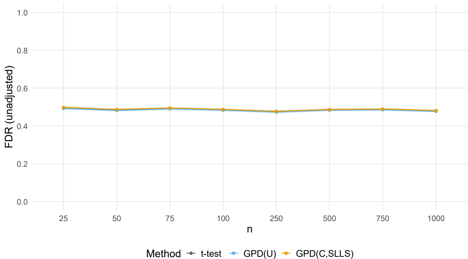
FDR (unadjusted) (alpha = 0.05)
