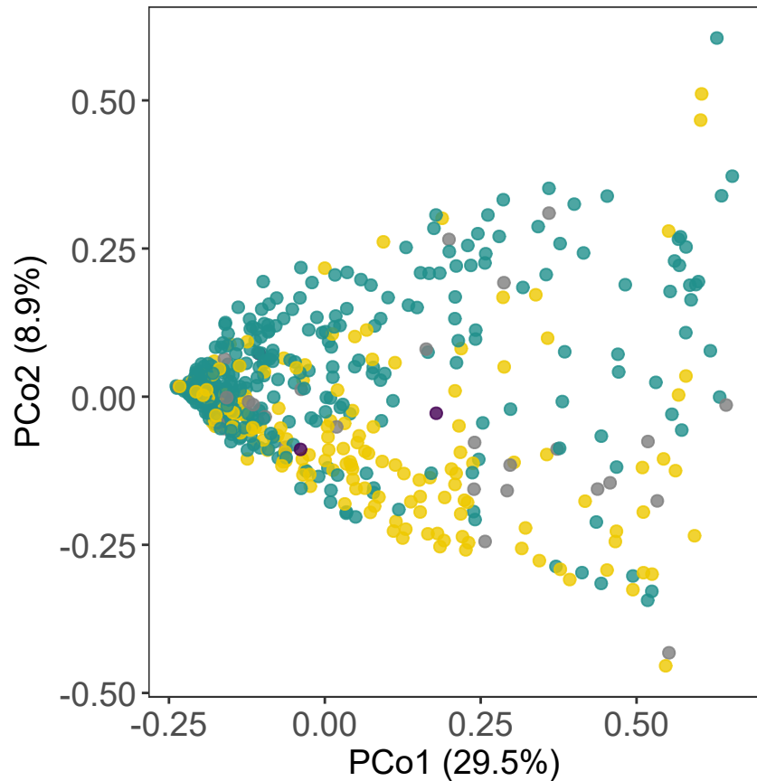
Bray-Curtis dissimilarity: EBF duration
