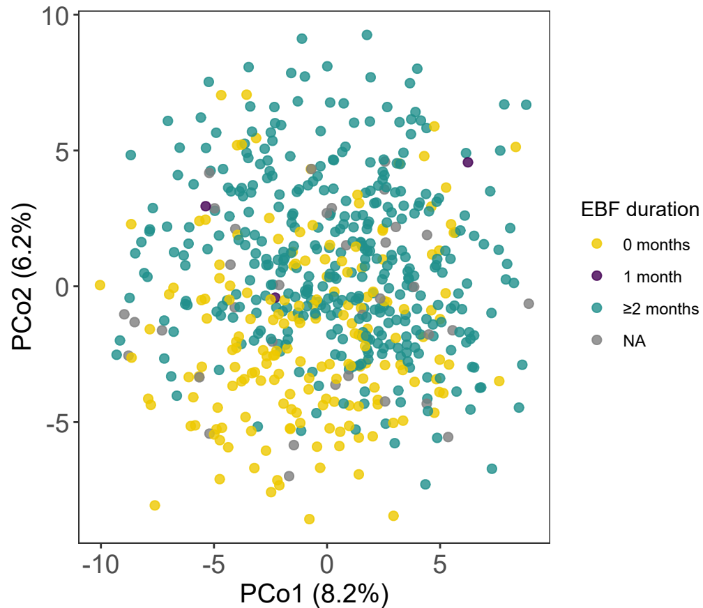
Aitchison distance: EBF duration
