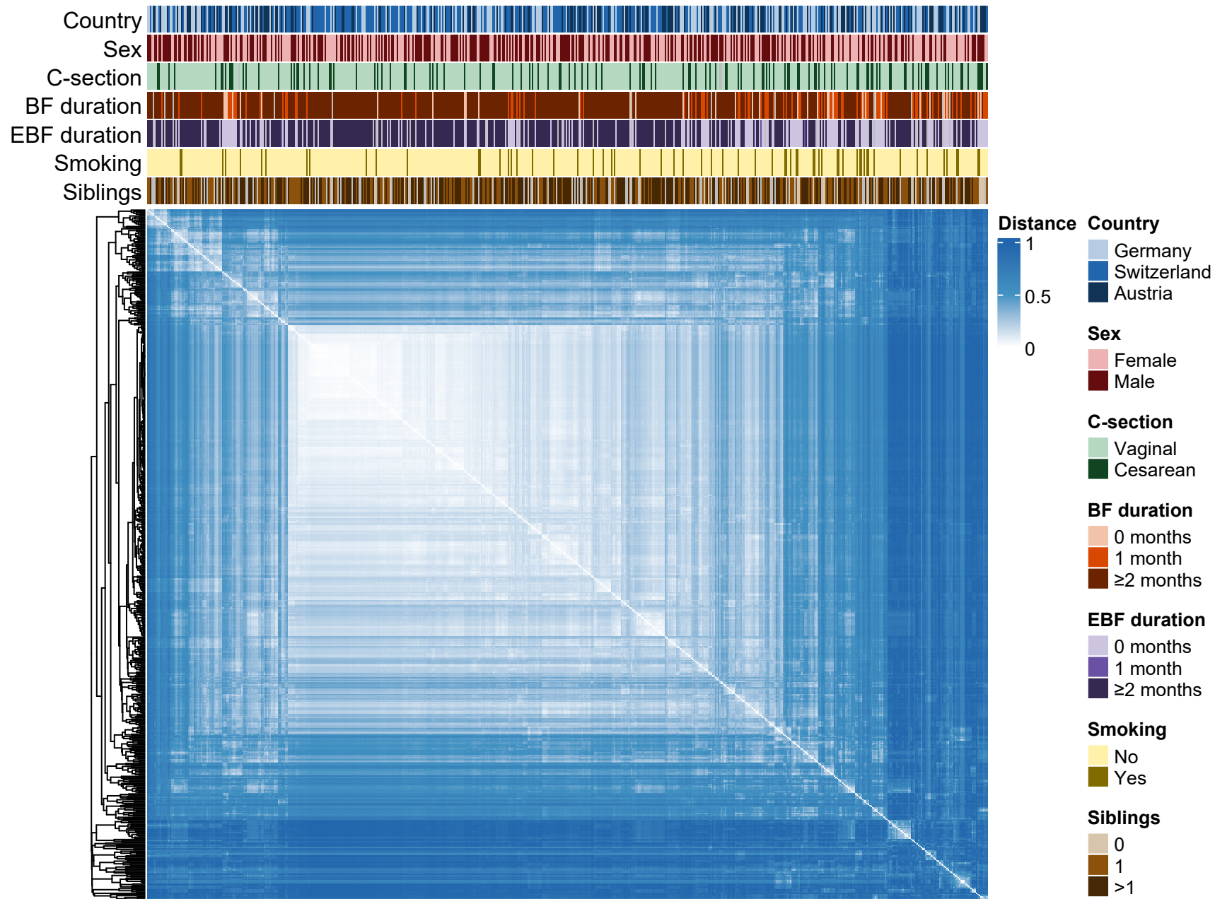
Bray-Curtis distance matrix
