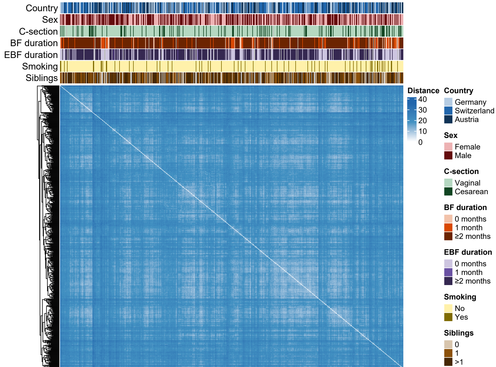
Aitchison distance matrix
