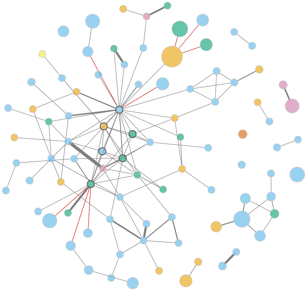
SPIEC-EASI MB (baseline network)
