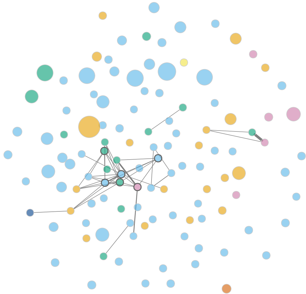
non-EBF
