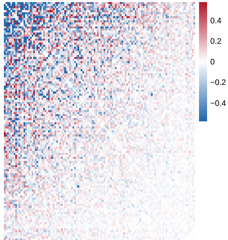
CLR inverse covariance
