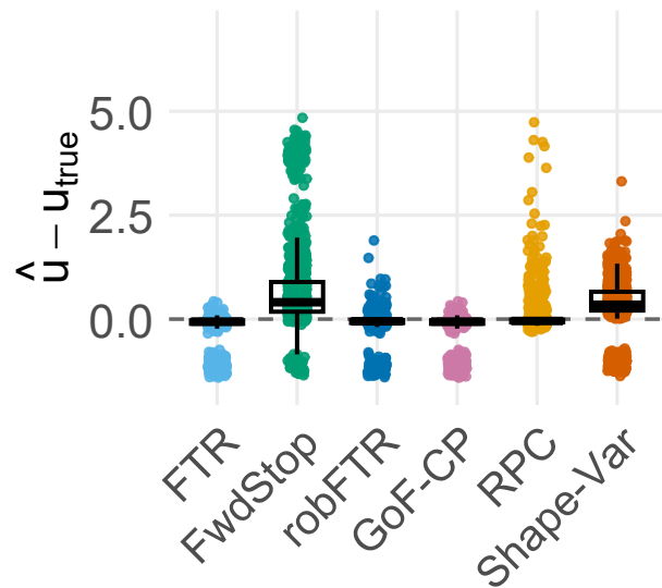
Weibull-GPD
