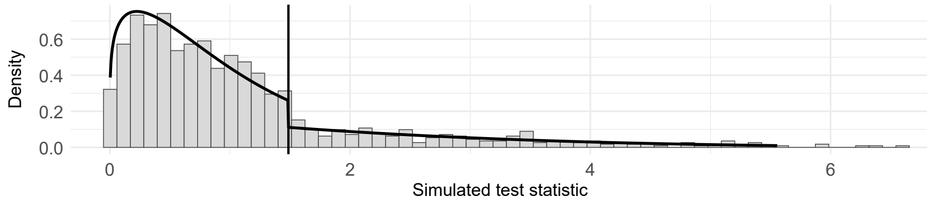
(b) Weibull-GPD ( k_0 = 1000 )
