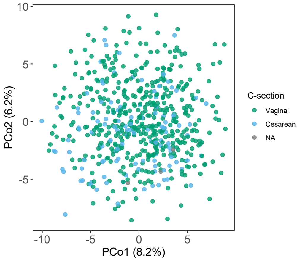
Aitchison distance: C-section
