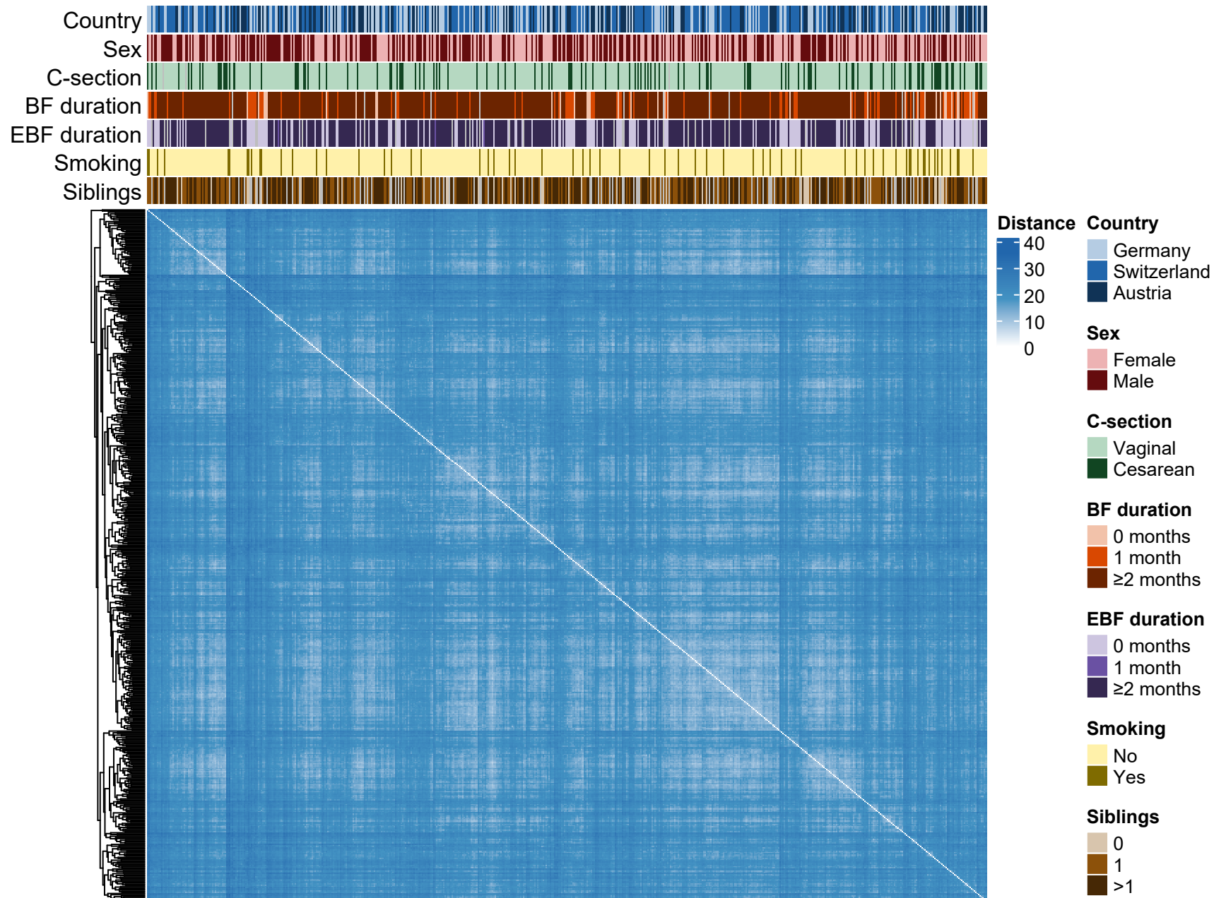
multRepl + CLR Euclidean distance matrix
